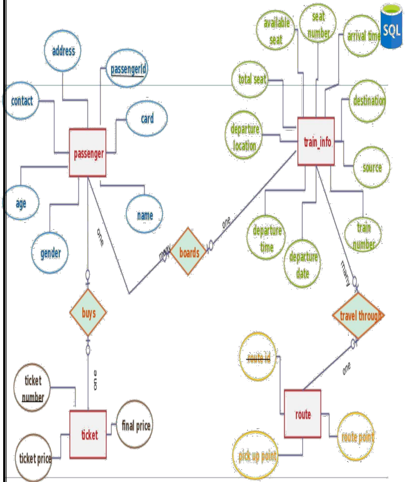
E R Model -(Railway Booking System)
